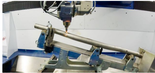
TruLaser Cell 8030 3D
