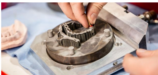
<p><span lang="EN-US">The telescopic crown is built up layer by layer from the powder bed. After this step, the crowns match the geometry of the primary coping almost perfectly, apart from a minimal amount that has to be milled off the inner surfaces. (Picture:</span> Steffen Müller-Klenk)</p>
